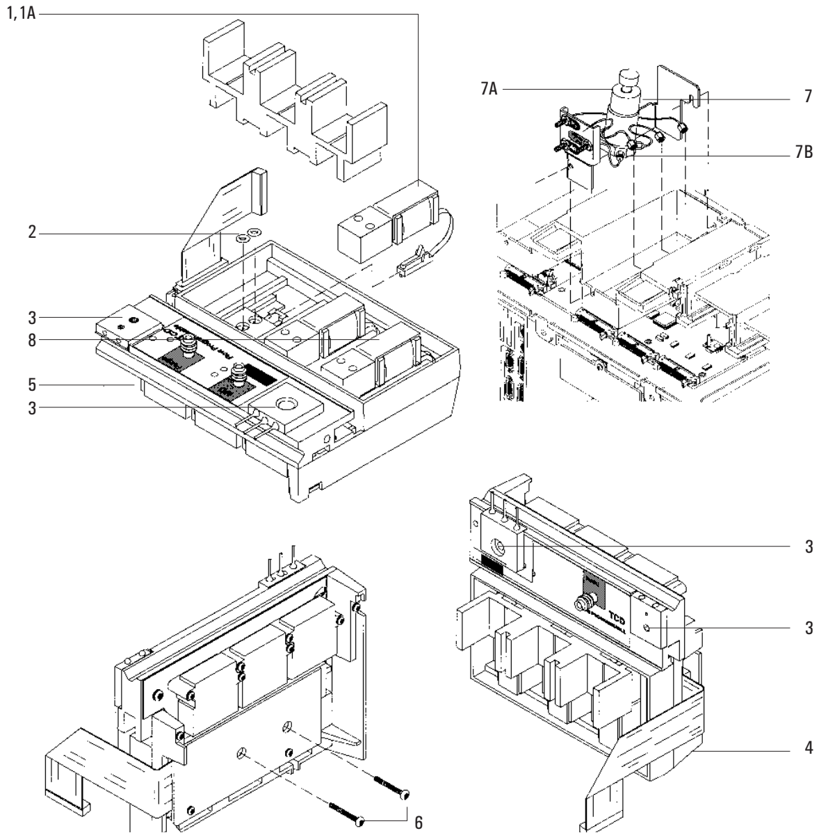
Figure 1320-8 (TCD) Manifold Assembly
